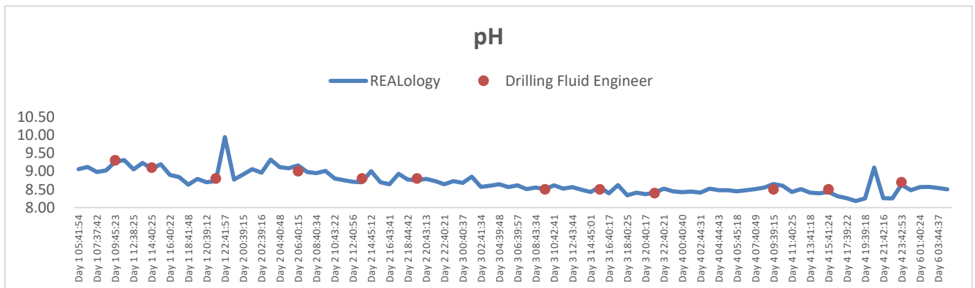
Fig2. Data indicates close trends between REALology and drilling fluid engineer data collation.
