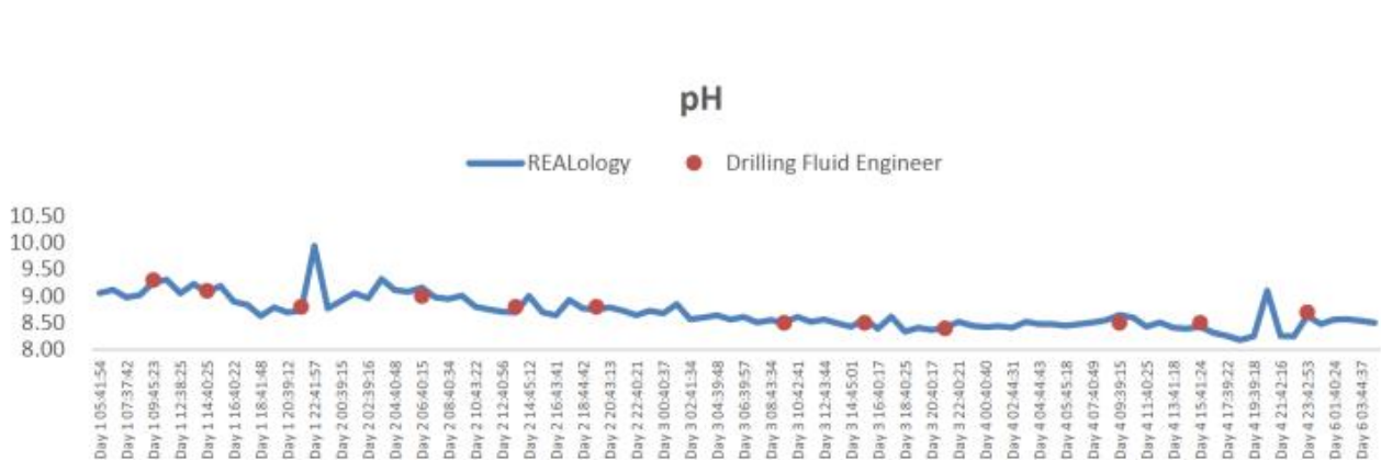
Fig2. Data indicates close trends between REALology and drilling fluid engineer data collation
