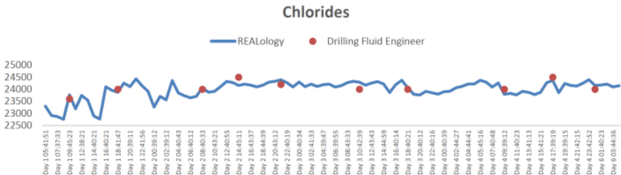
Fig3. Result indicates deviation between REALology and manual test data < 3%
